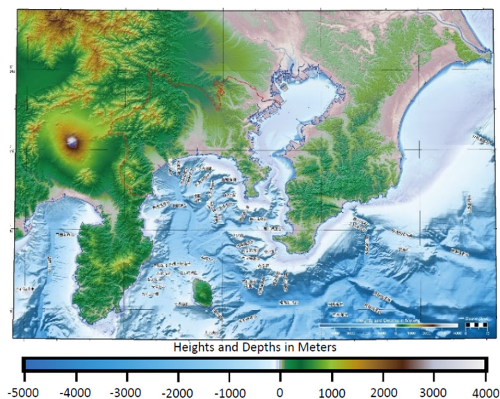
Figure 40: Topographic map of Sagami Bay and Sagaminada seafloor
