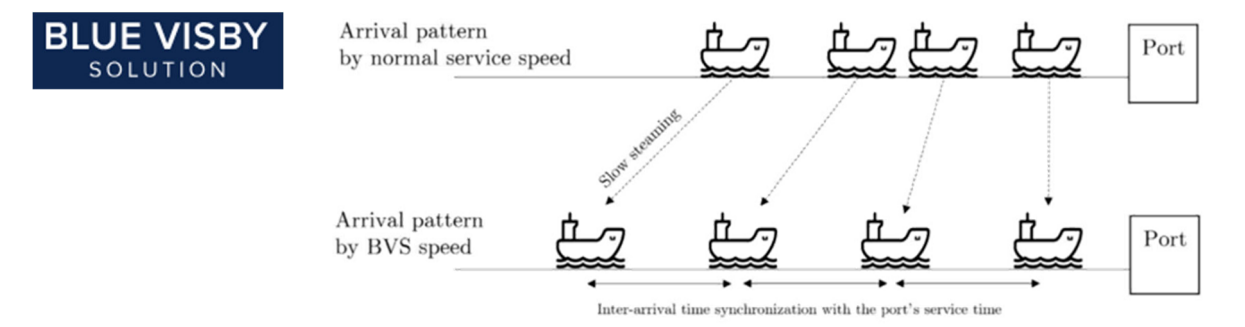
Figure 22: Optimization and dispersion of arrival times for groups of vessels heading for the same port
